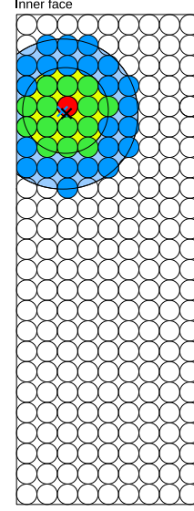
Figure 5.15: PMT selection used in the position fitting. The blue cross marker shows the initial estimate of interaction point calculated by the weighted mean around the maximum output PMT shown as red color. The PMTs used in the first fitting are those within 3.5-PMT distance from the point. The second fitting is done in more restricted region, 2-PMT radius shown as green PMTs from the result of the first fitting shown as black cross.
