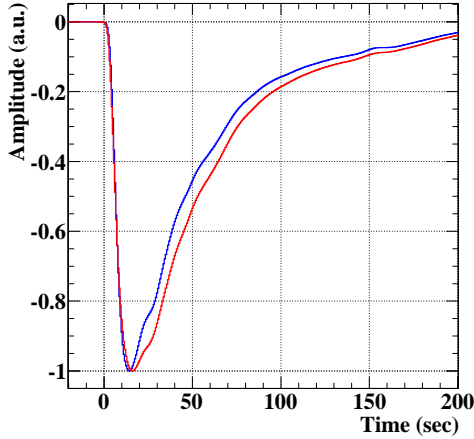
Figure 6.16: Change of LXe pulse shape. Blue line shows the average pulse shape at the beginning of run 2008 (in September), and red one shows that at the end of the run (in December). Those two are normalized by the pulse heights.
