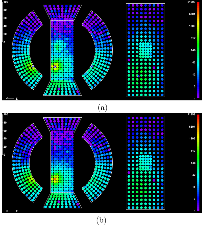
Figure 5.20: Light distribution before(a) and after(b) eliminating pileup contribution. The color axis shows the amount of observed light on each PMT.
