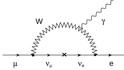
Figure 2.1: Example of Feynman diagram describing the \mu \rightarrow e\gamma decay in the SM with a neutrino-mass extension.
