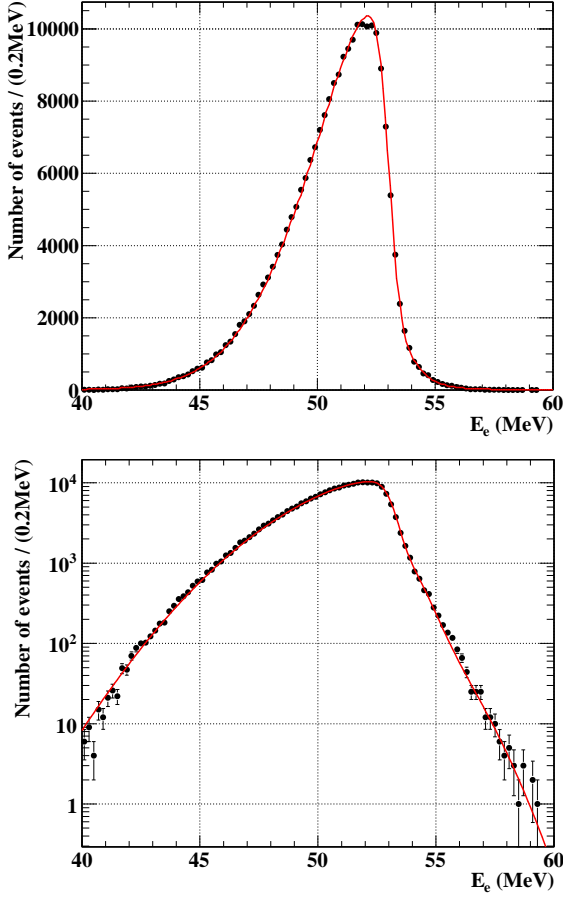
Figure 8.6: Positron background spectrum. Black circle plot shows data spectrum measured in the sideband. Red solid line shows Michel spectrum folded with acceptance and efficiency function and detector response fitted to the data.
