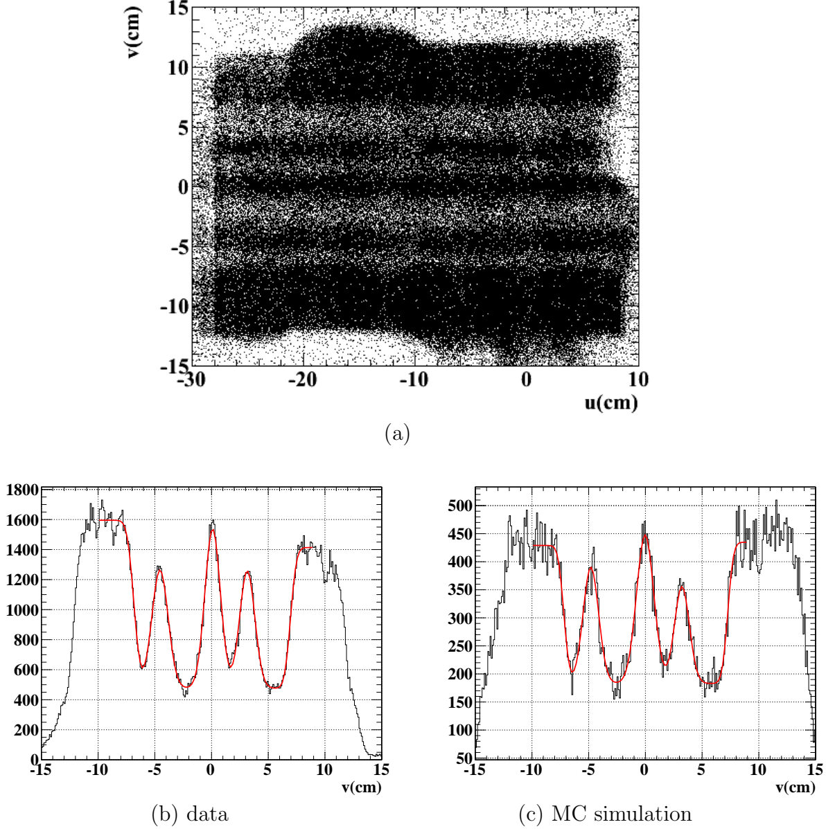
Figure 7.15: Event distribution of \pi^0 run with a Pb brick. (a) shows scatter plot of the reconstructed position of the data. (b) shows the projection on v -axis for the data, and (c) shows that of the MC simulation.
