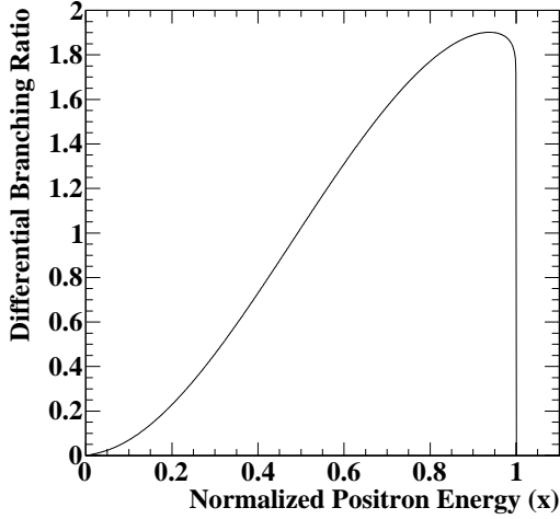
Figure 2.9: Positron energy spectrum of unpolarized \mu^+ \rightarrow e^+ \nu_e \bar{\nu}_\mu decay (Michel spectrum). A radiative correction due to the virtual photon emission and the inner bremsstrahlung is applied in the spectrum [36].
