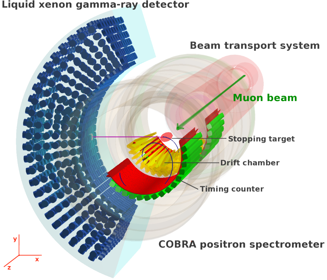
Figure 3.1: Overview of the MEG experiment.
