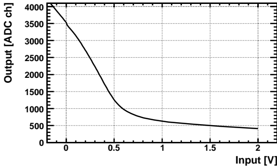
Figure 6.1: Typical response curve of a DRS cell.
