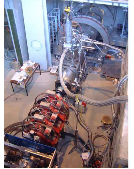
Figure 3.4: Schematic and picture of beam transport system. Surface muons enter from the left and go through the Wien filter, the BTS, and the COBRA magnet to reach the stopping target at the center of the magnet.
