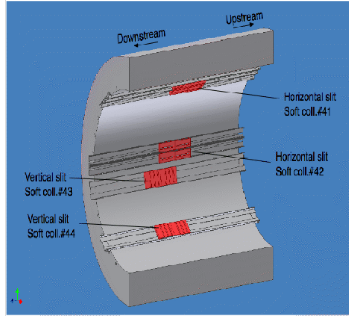
Figure 4.3: Configuration of lead bricks installation.
