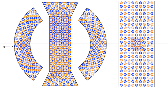
Figure 7.20: PMT grouping scheme for the intrinsic time resolution study. PMTs indicated with blue circles belong to odd group, and those with orange circles belong to even group.
