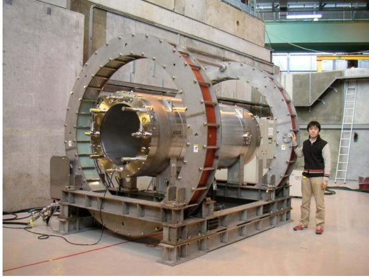
Figure 3.9: Picture of the COBRA magnet.
