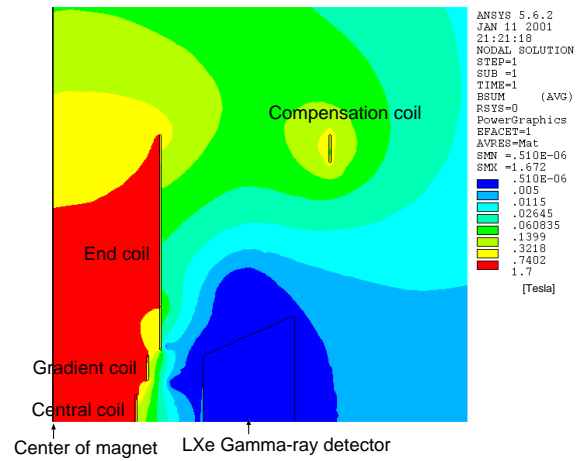
Figure 3.13: Contour plot of fringe field around the gamma-ray detector.
