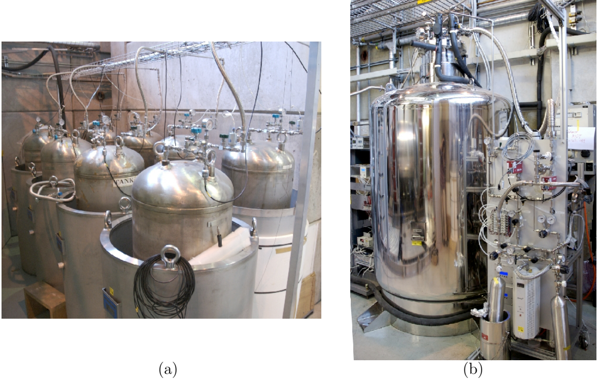
Figure 3.28: Pictures of xenon storage systems. (a) eight high-pressure gas storage tanks. (b) 1000 liter liquid storage dewar.
