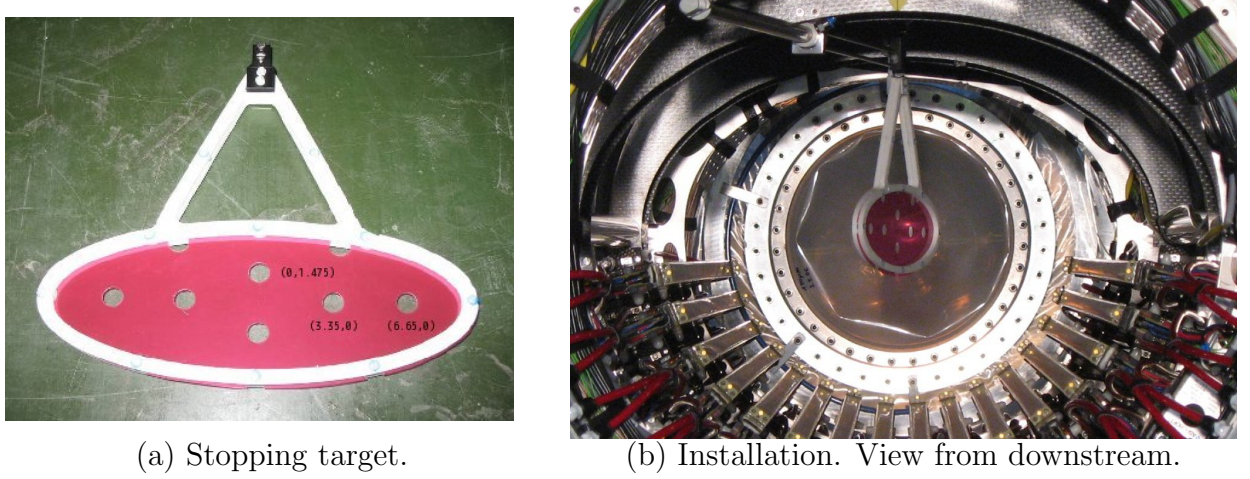
Figure 3.5: Pictures of MEG stopping target.
