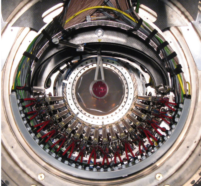
Figure 3.14: Picture of drift chamber system inside the COBRA magnet.
