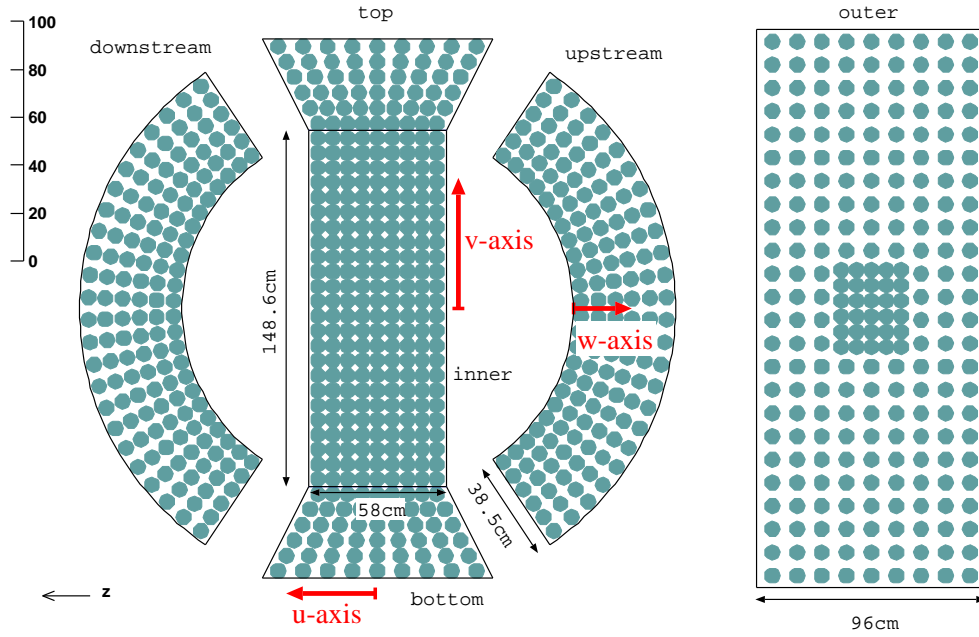
Figure 3.25: Development view of LXe gamma-ray detector. The local coordinate system of the detector is also shown as red arrows. Each light blue circle shows a PMT.
