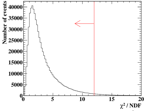
(a) Distribution of normalized \chi^2 .
