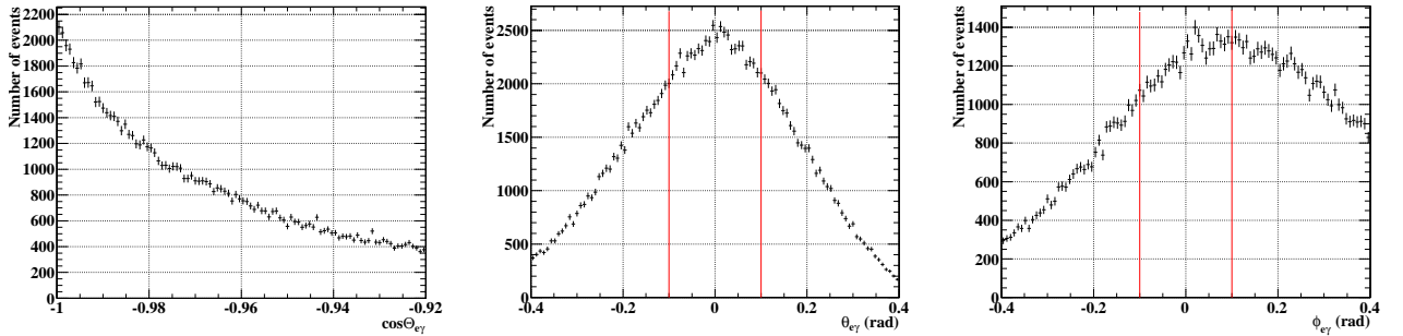
Figure 8.8: Angular distributions of background in the sideband.
