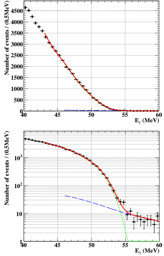
Figure 8.7: Gamma background spectrum. Black circle plot shows data spectrum measured in the sideband data. Red solid line shows the MC spectrum folded with detector resolution fitted to the data. The MC spectrum is composed of single-gamma component (green dotted line) and pileup component (blue dashed line).
