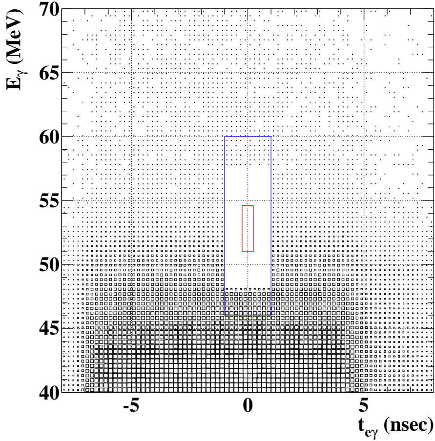
Figure 8.1: Distribution of t_{e\gamma} v.s. E_{\gamma} after the pre-selection and blinding process. No cuts are applied. Events outside the pre-selection time window come from accidental overlap positrons. Analysis window for the likelihood analysis and signal box (A) are also shown as blue and red boxes, respectively.
