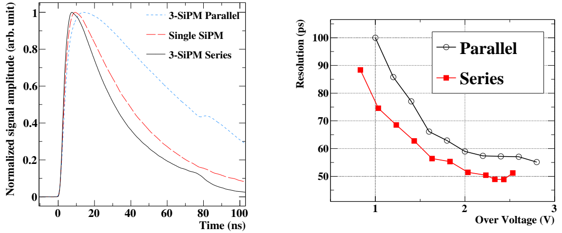
Figure 4.12: Connection comparison with test counter made from 60 \times 30 \times 5 mm 3 BC422 scintillator attached 3 Hamamatsu Photonics SiPMs (S10362-33-050C). Averaging waveforms with several thousand events are shown in left figure [32]. They are normalized by their amplitudes. The resolution comparison between parallel and series connections is in right figure in which over voltage is written as that for one SiPM.
