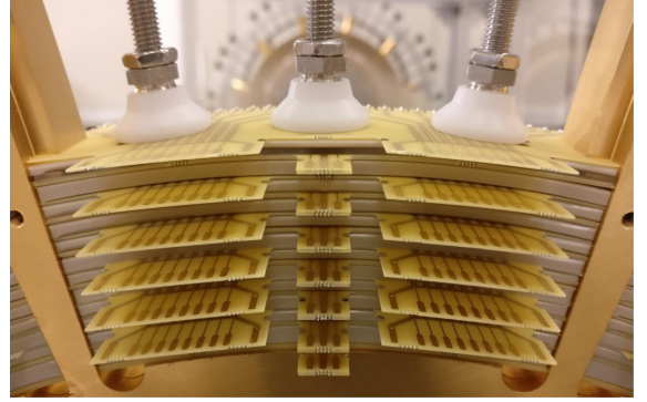
Figure 3.29: Picture of end-plate with PCB and spacer during wiring each layer by using fixing tool shown in top of the picture.
