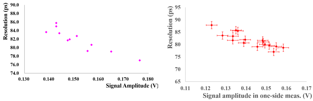
Figure 4.28: Resolution and amplitude of the counters with several SiPM array Figure 4.29: Correlation between signal amplitude from the one-side measurement and the resolution.
