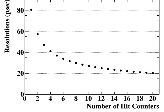
Figure 4.7: Overall resolution as a function of number of hit counters
