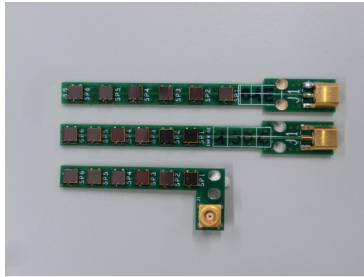
Figure 4.23: PCBs for SiPM arrays. Three types are prepared for 5 cm height (top), 4 cm height (middle), and L-shape (bottom)
