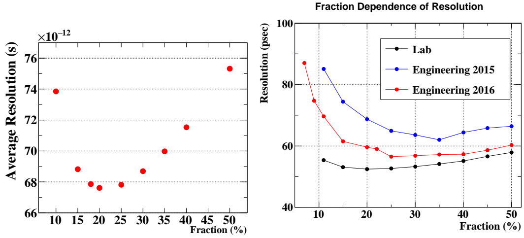
Figure 7.10: Resolutions with several fraction for the waveform analysis in pilot run 2015, 2016 and pre-test with ^{90}\text{Sr} source. Expected resolution decreasing from energy deposit point of view is 5-10 %.
