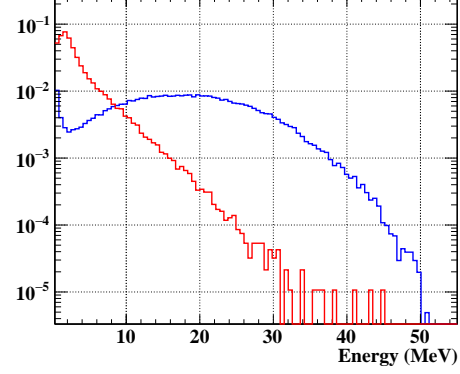
Figure 3.47: Expected energy distribution in RDC from RMD positrons which photon energy is more than 46 MeV (red) and Michel positron (blue).
