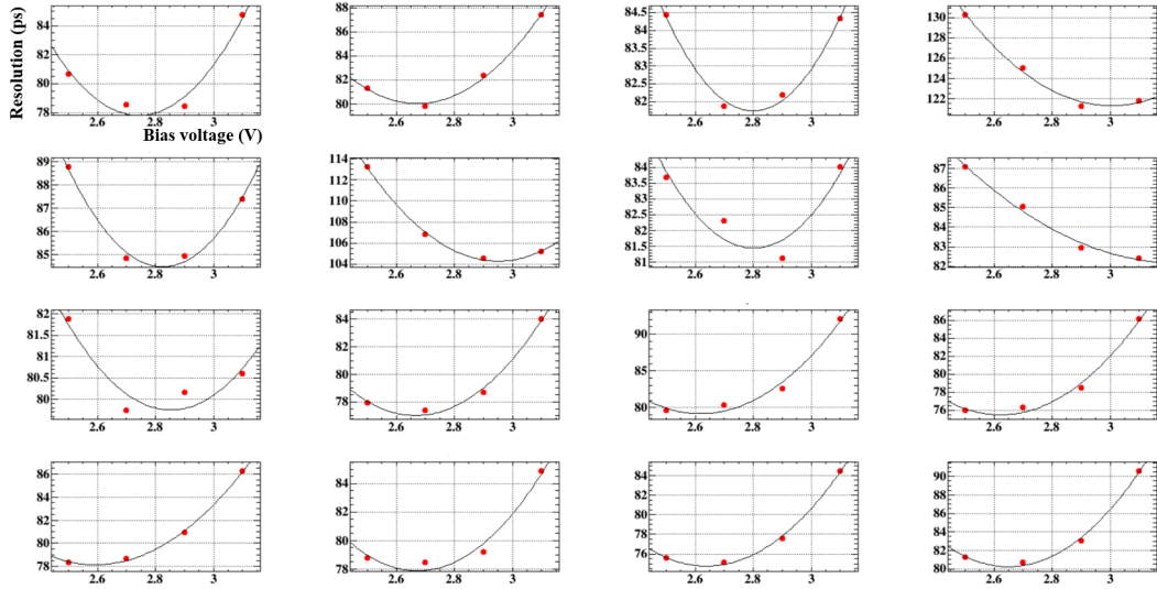
Figure 4.26: The resolution dependence on bias voltage of Type 1 SiPMs. They are fit with a \times (v - p)^2 + q where v is over voltage.
