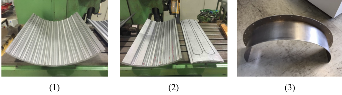
Figure 4.52: Picture of support frame. (1) Middle part ( < \phi < ) in main part of the frame. (2) Smaller (right) and larger (left) \phi part ( \phi and \phi ). Small \phi part is turned over. The backside has groove for cooling pipe. (3) Frame for COBRA inner counters.
