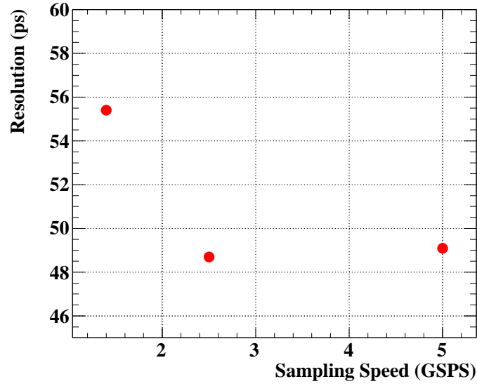
Figure 4.47: Resolutions dependence on sampling speed.
