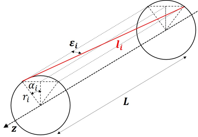
Figure 3.30: Schematic of stereo angle ( \epsilon_i ) of wire in i th layer. L is DCH length; l_i wire length; \alpha_i angle projected to end-plate; and r_i radial position of a wire
