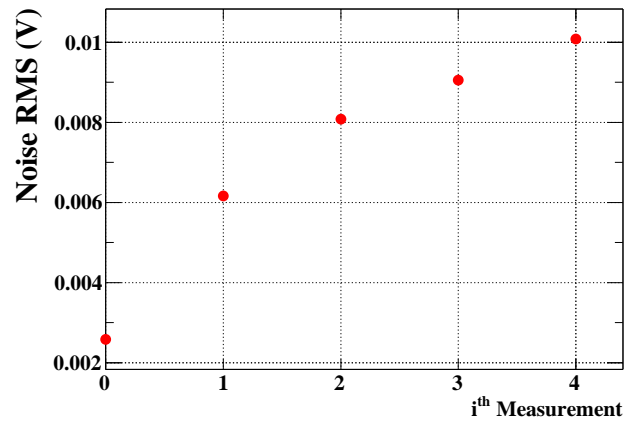
Figure 4.43: Noise level with irradiation.
