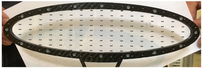
Figure 3.16: Target in MEG. There are six holes for vertex study and for monitoring target alignment.
