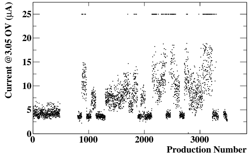
Figure 4.22: Current at OV 3.05 V. Saturated point of the IV measurement is 25 \mu\text{A} .
