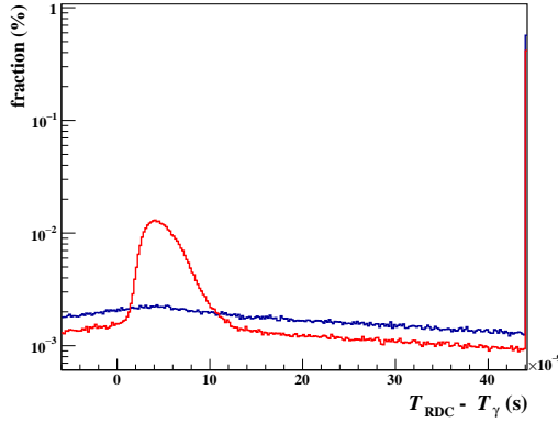
Figure 3.46: Distribution of relative time between the RDC and the LXe detectors in MC. Time resolution of 100 ps is assumed.
