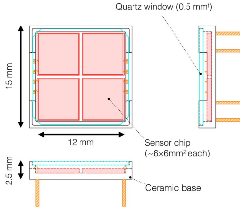
Figure 3.43: Drawing of SiPM for LXe.
