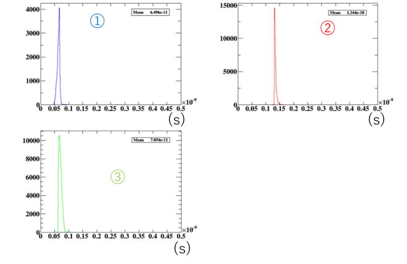
Figure A.1: TOF distributions for each hit pattern.
