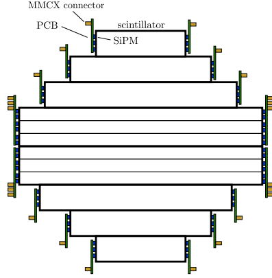
Figure 3.49: Schematic view of scintillator bar attached SiPMs for time measurement.
