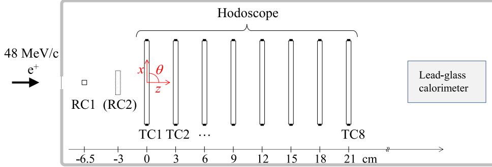
Figure 6.1: Set up in the beam test in Frascati.
