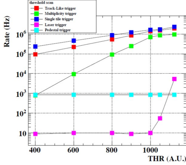
Figure 7.5: Scanning of discriminator threshold. Laser is flushed at 10 Hz. The threshold setting parameter has an offset. Higher value means lower threshold.
