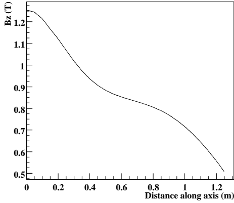
Figure 3.23: Profile of the COBRA magnetic field.
