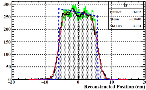
Figure 5.8: The distribution of the hit position on a counter. The green line show the original distribution and the black is after taking moving average. By convolving a trapezoid (blue and red lines) with Gaussian, the distribution of the hit position is fit.
