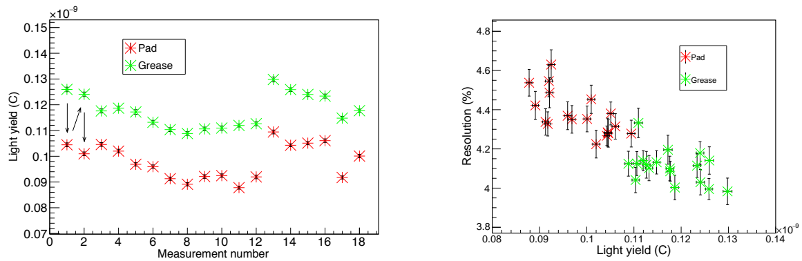
Figure 4.18: Comparison of the grease and the pad. Left : Comparison of the light yield. The arrows represent the order of the measurement. Right : The energy resolution and the light yield.
