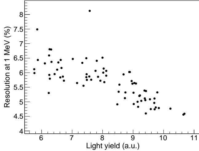
Figure 4.3: Distribution of the light yield and energy resolution.
