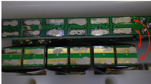
Figure 5.27: PCB (top) and SiPMs (bottom) after disassembling. The red arrows show the glued areas before disassembling.
