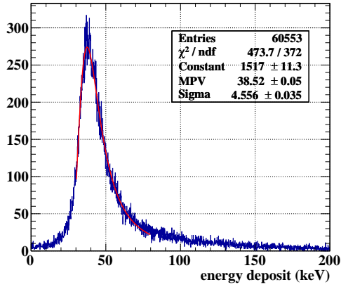
Figure 6.21: Simulated energy deposit of the positrons from RMD ( E_\gamma > 48 MeV).
