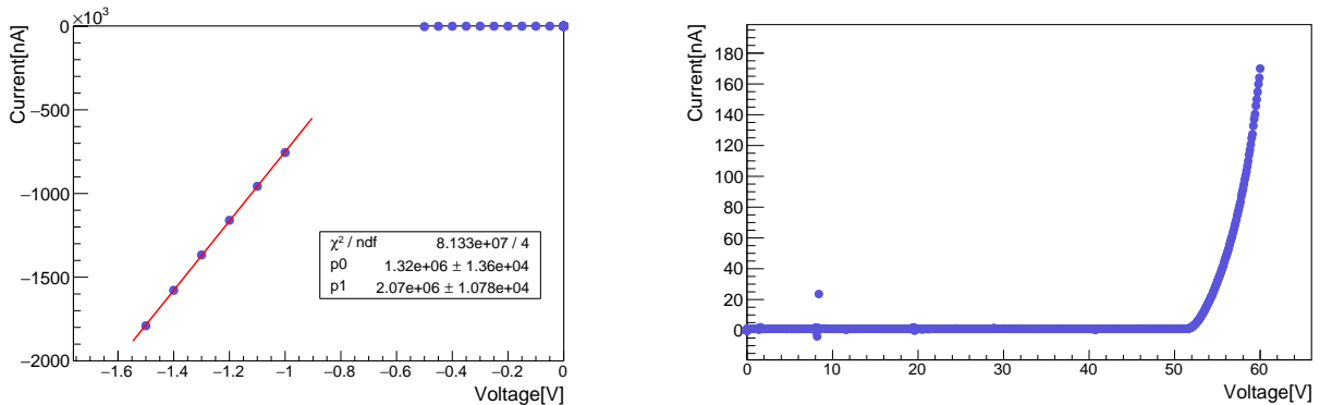
Figure A.3: I-V curve of the SiPM. Left : Negative bias voltage. Right : Positive bias voltage. Due to the current limitation, we did not use the software below -1 V, but we read the value on the display of the picoammeter.
