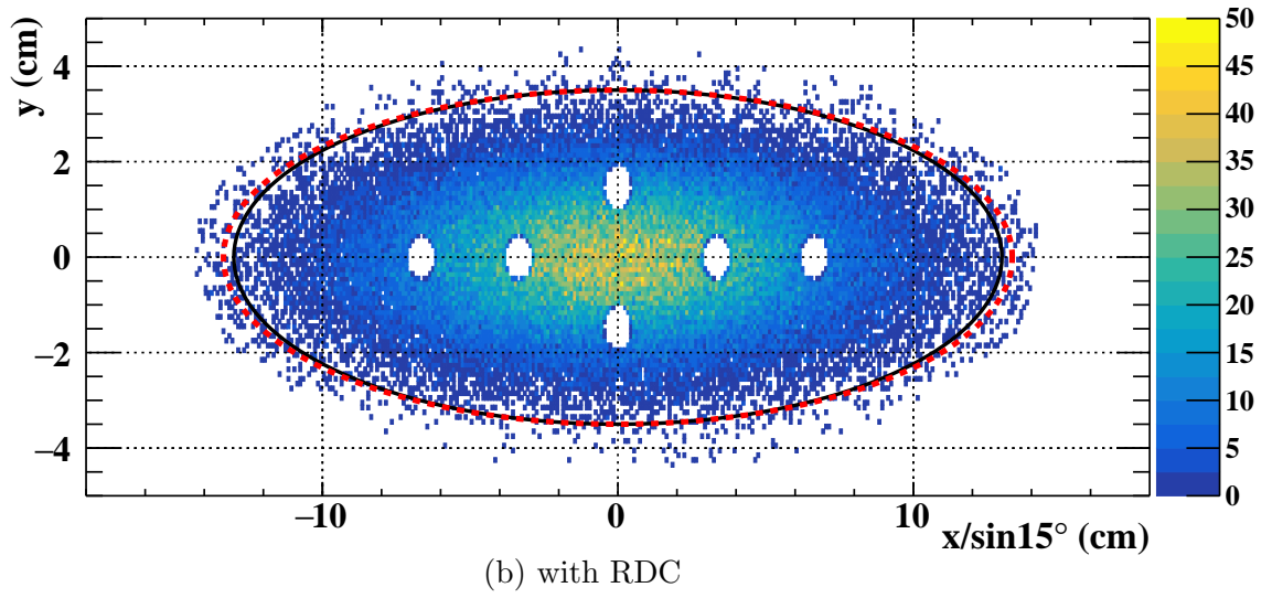
Figure 6.3: Distribution of the muon vertex on the target. Black solid line and red dashed line represent the fiducial area of the nominal and bigger target, respectively.
