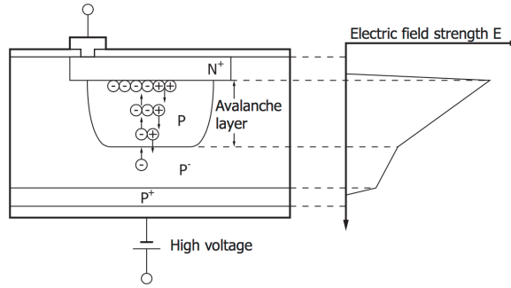
Figure A.2: Schematic diagram of avalanche multiplication [23].
