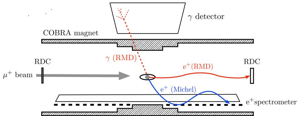
Figure 3.1: Schematic view of MEG II detectors
